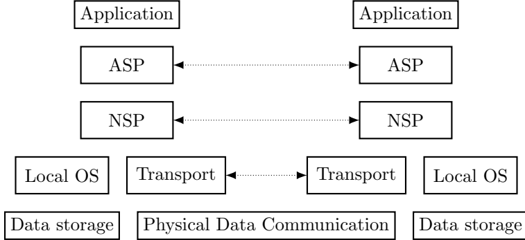
Figure 10: Relationships between synchronization components.
