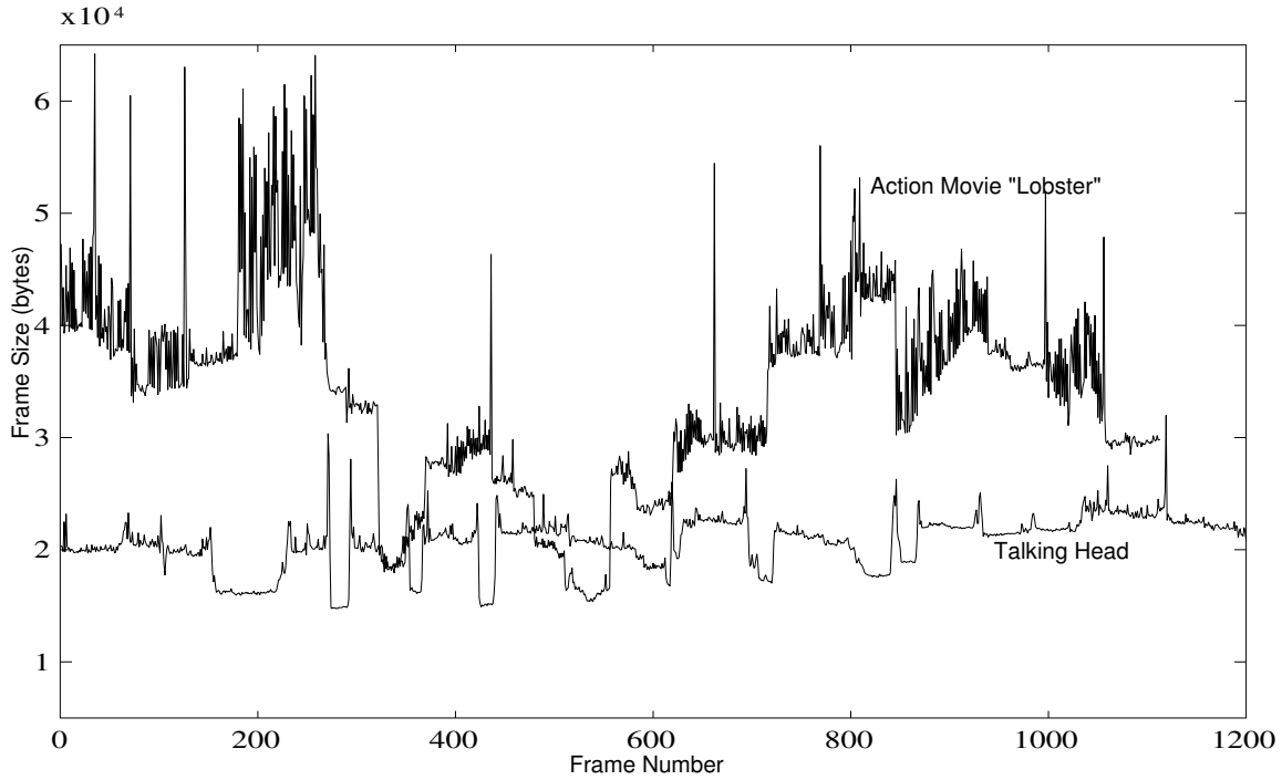
Figure 7: Image Size Dynamics for JPEG-Compressed Movie
