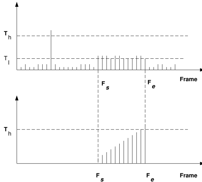
Figure 9: Illustration of Twin-Comparison
