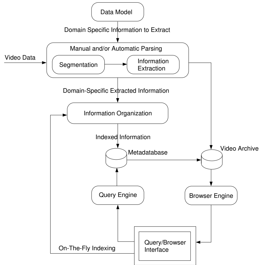
Figure 2: Processes for Construction and Use of a Digital Video Library
