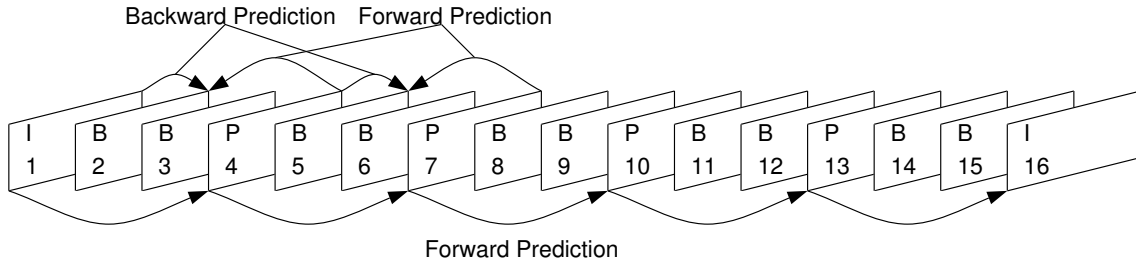
Figure 11: A Typical MPEG Compressed Video Sequence
