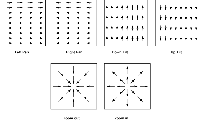
Figure 10: Optical Flow Field Produced by Pan, Tilt and Zoom
