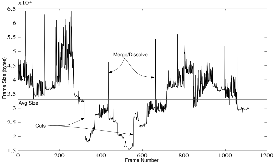
Figure 8: Illustration of Various Scene Transitions
