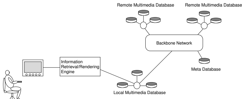
Figure 1: Distributed Databases
