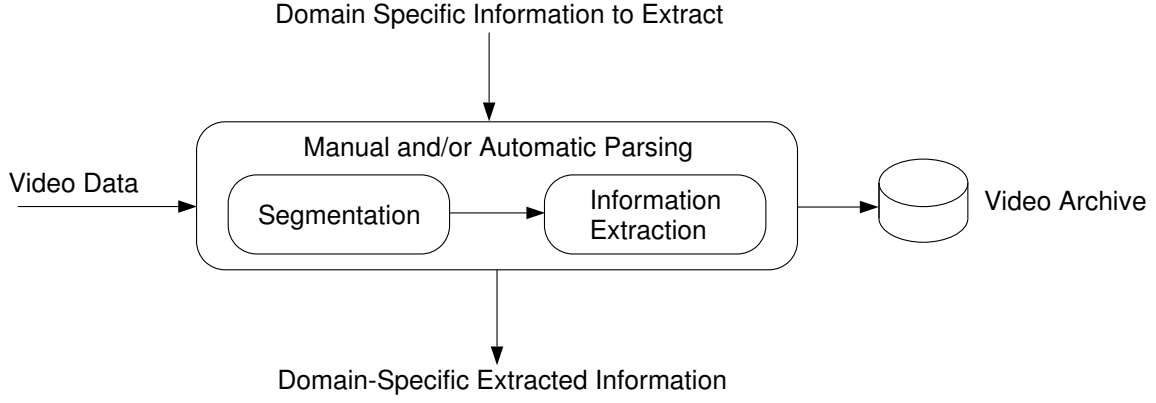
Figure 6: Second Stage in Video Data Adaptation: Information Extraction
